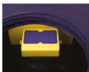
Anti-foam system with vacuum motor protection
